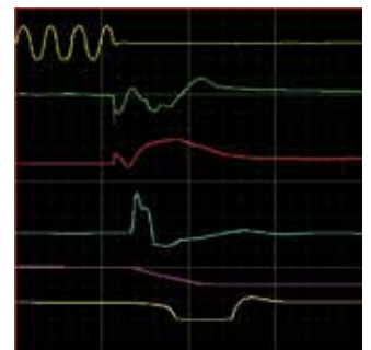
● Battery evaluation (Example measurement of control signal and charge/discharge time)
